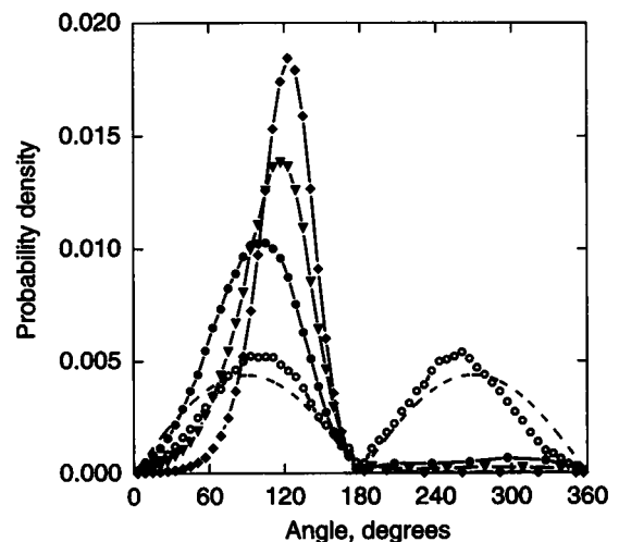
FIGURE 6 The angular distribution between juxtaposed segments of circular relaxed and supercoiled DNA. The angle between all segments within 10 nm of each other but separated by more than 1 kb along the DNA contour was calculated. The data were computed for a circular DNA 3.5 kb in length that was either supercoiled ( \sigma of -0.01 (●), -0.03 (▼), -0.05 (◆)) or relaxed (○). For comparison, the distribution for random vectors is shown by the thin dashed line.
